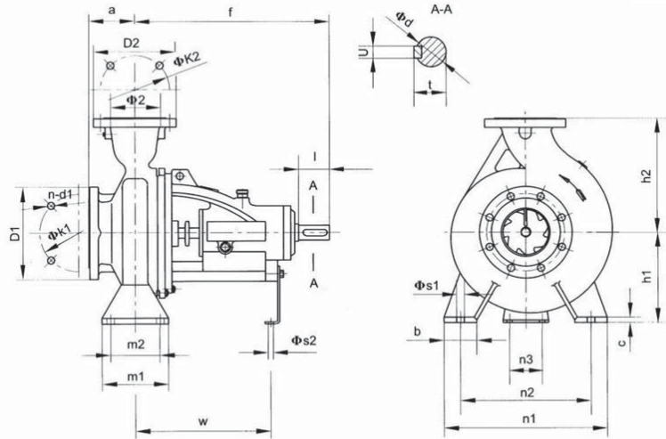
Overall and Mounting Dimensions
